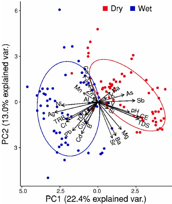
Fig. 2. Distribution of physicochemical parameters, metals and metalloids in dry (2017) and wet season (2018).
